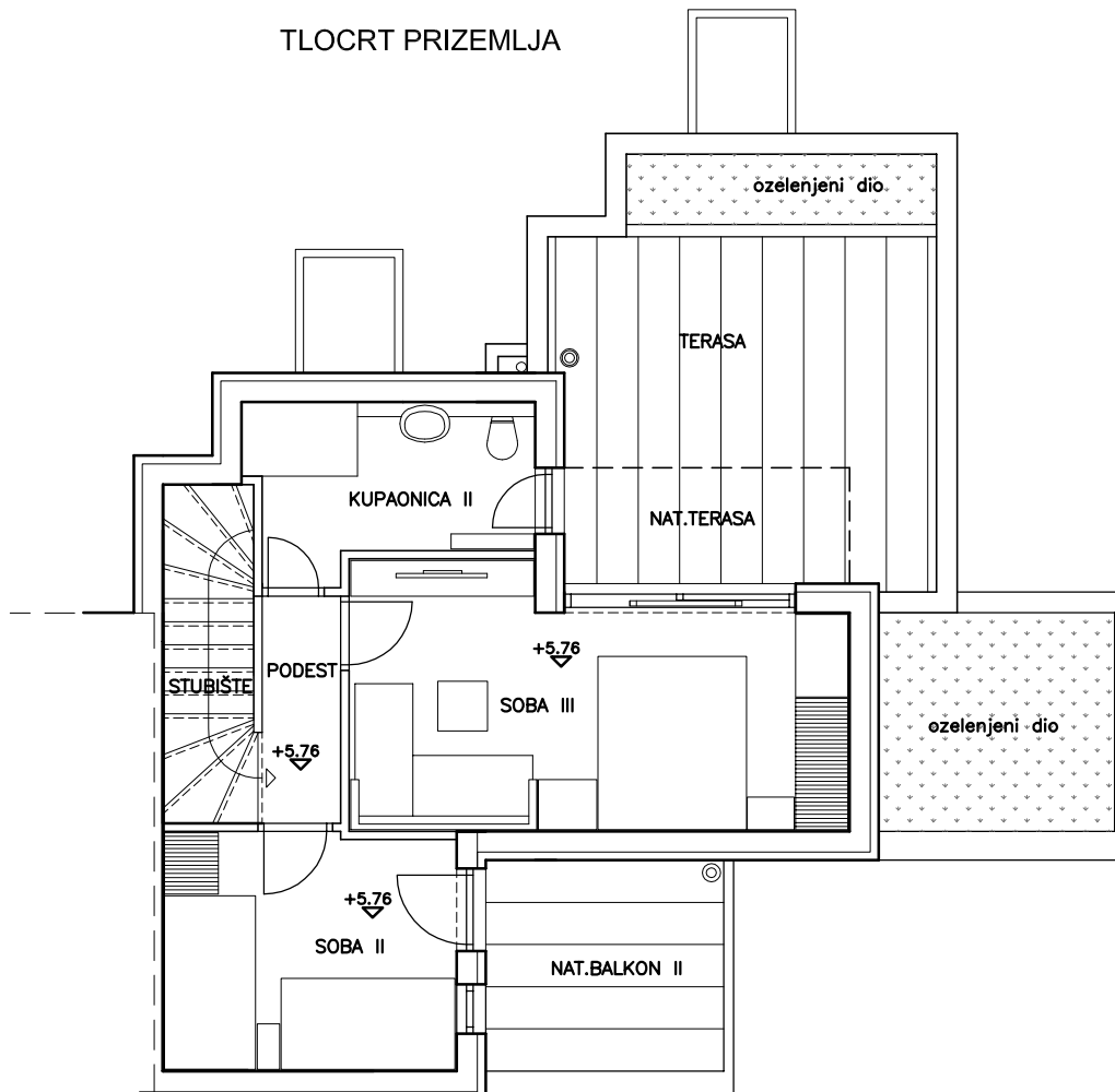
TLOCRT II.KATA
